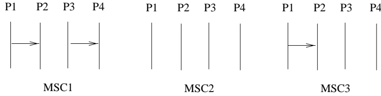
Fig. 7. Safe realizability is not entirely captured by CC3
