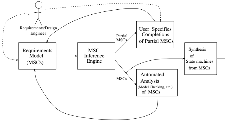
Fig. 11. Using the MSC inference framework
