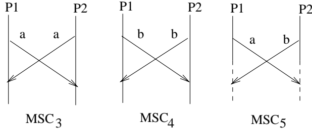
Fig. 5. Weakness of weak realizability
