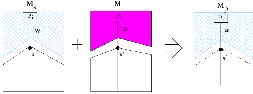
Fig. 9. Inference algorithm illustration
