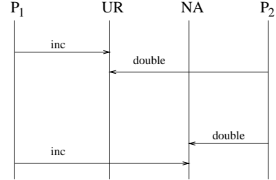
Fig. 2. Implied MSC bad : Incorrect fuel mix
