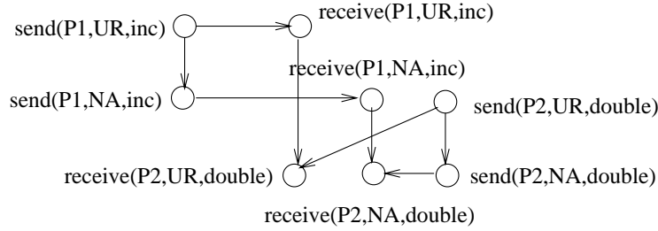
Fig. 3. Partial order representation of MSC_1
