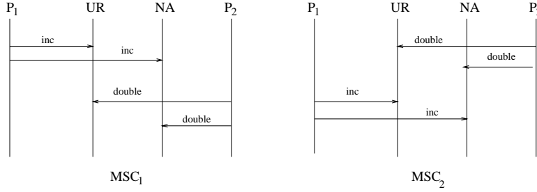
Fig. 1. Two seemingly “correct” scenarios, updating fuel amounts
