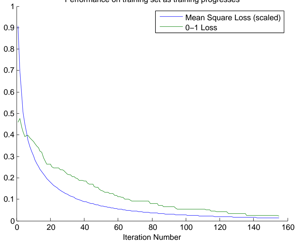
Performance on training set as training progresses
